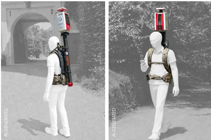
RIEGL VZ-600i kinematic data acquisition using a RIEGL VZ-i Backpack Mount
