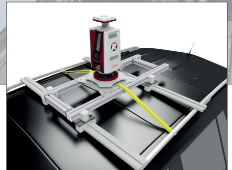
RIEGL VMY/VMX Roof Mount
