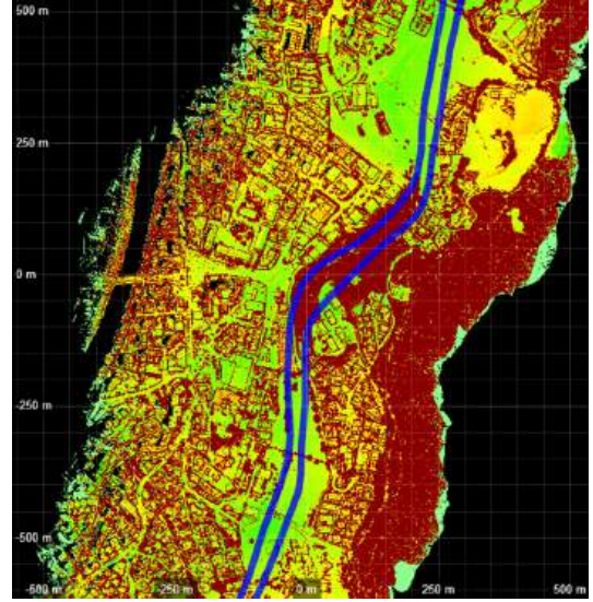
(a) Strip differences for all G/I point clouds (both passes).
