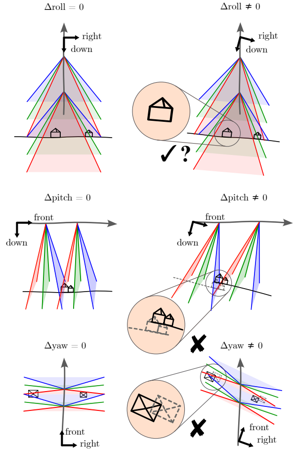
Figure 4. Point cloud discrepancies caused by orientation errors ( \Delta\text{roll} , \Delta\text{pitch} , \Delta\text{yaw} ) with NFB scanning. The left side shows the NFB scan geometry with no orientation errors, the right side for non-zero roll, pitch or yaw error.
