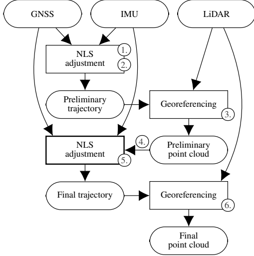
Figure 1. Trajectory Estimation and Georeferencing workflow from Pöpl et al. (2025).
