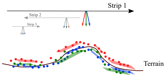
Figure 3. Trajectory errors cause discrepancies in overlapping point clouds originating from different strips or views. Planar features are extracted and then matched with each other.
