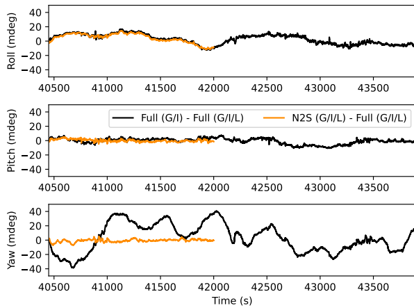
Figure 9. Difference between full G/I trajectory and full G/I/L trajectory, and between north-to-south G/I/L trajectory and full G/I/L trajectory.
