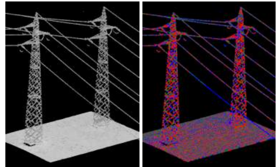
Figure 8. Point cloud of power line and pylon, colored by reflectance (left) and scan direction (right).
