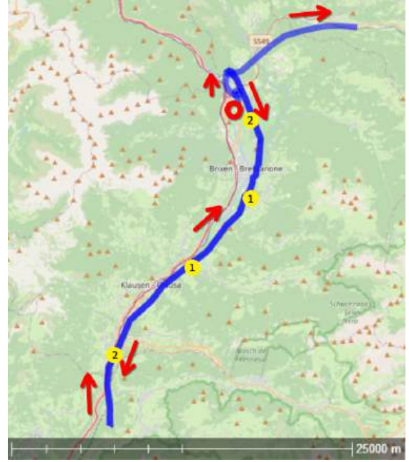
Figure 6. Data acquisition flight path. The helicopter took off at the airfield marked with a circle and, after a short initialization maneuver, mapped 30 km of overhead power line in two passes. The final portion of the flight, east towards a different airfield, is not used. Reference surfaces (6 surfaces at 4 sites) are marked in yellow.
