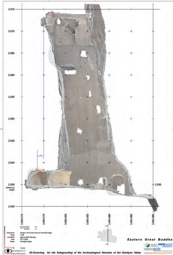
Fig. 5. Orthophoto generated from the laser scan.
