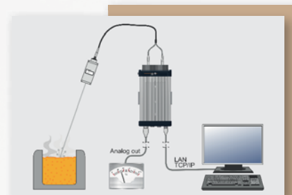
Level Measurement of Liquid Steel in Melting Pots
