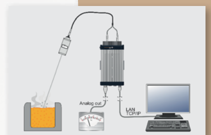
Level Measurement of Liquid Steel in Melting Pots
